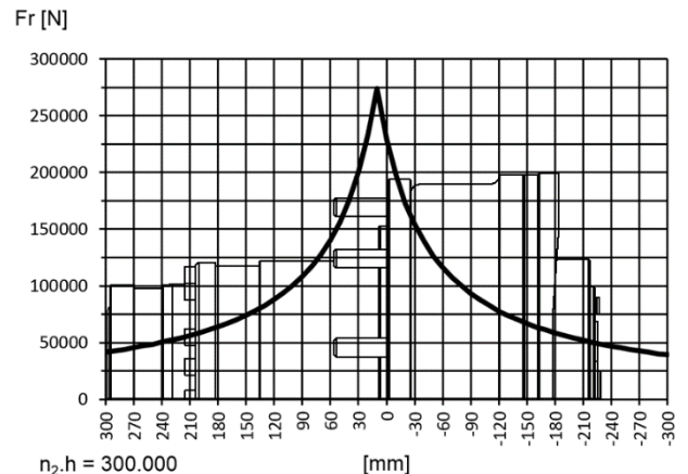
RADIAL LOAD
