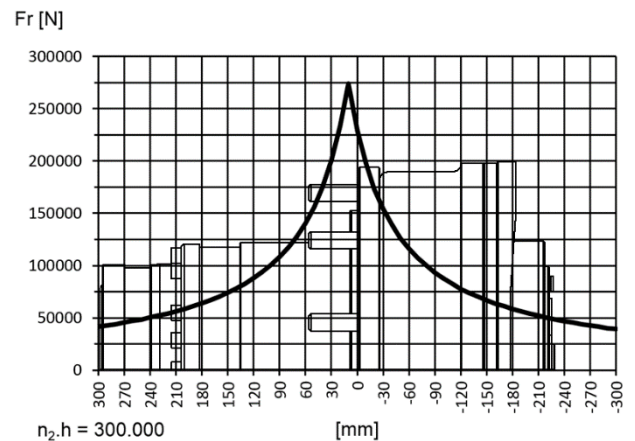
RADIAL LOAD
